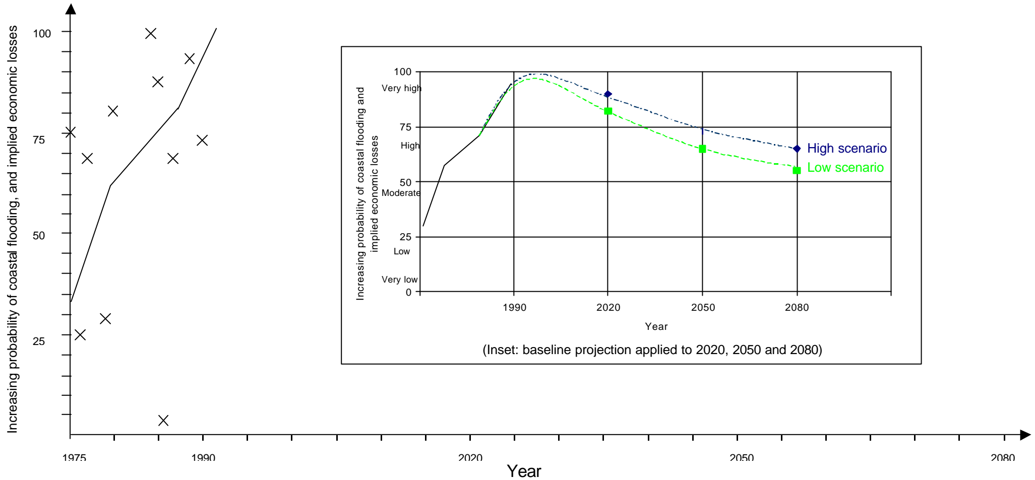
Figure 5.A-6. Baseline projection, probability of coastal flooding and implied increase in financial losses
